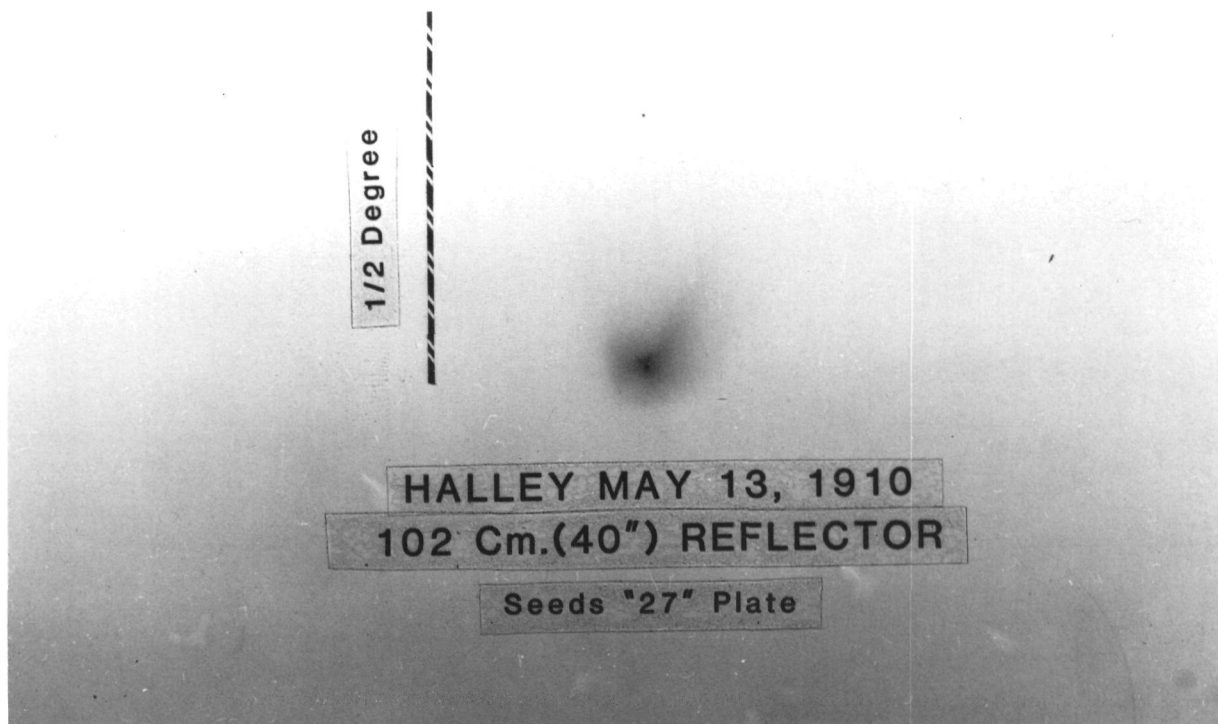
Figure 1. Direct photograph of the head region of Comet Halley 1910II on May 13, 1910.
